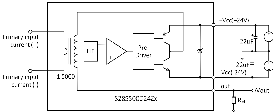
Fig3. Block diagram
